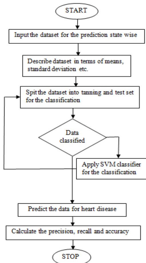
Figure 1: Proposed Flowchart
