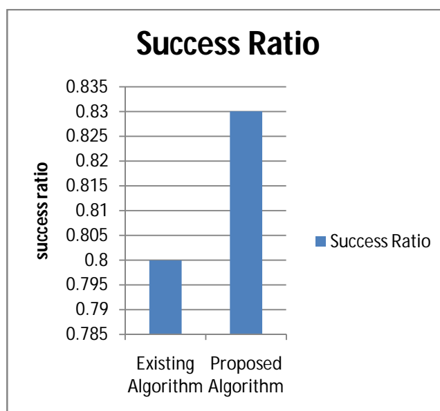
Fig 3: Success Ratio
