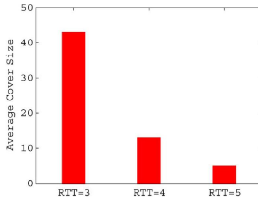
Fig 3. Algorithm coverage for different RTT values.
