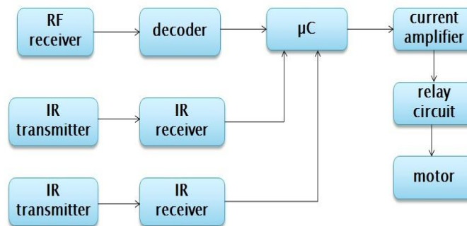
Fig.3 Block diagram of the working vehicle
