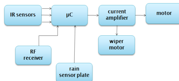
Fig.1 Generic Block Diagram
