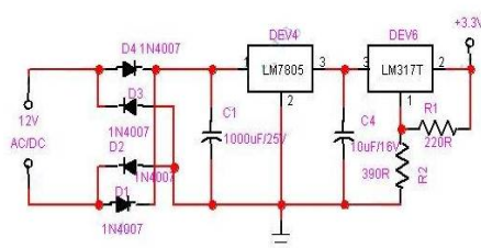
Figure 2. Supply Circuit
