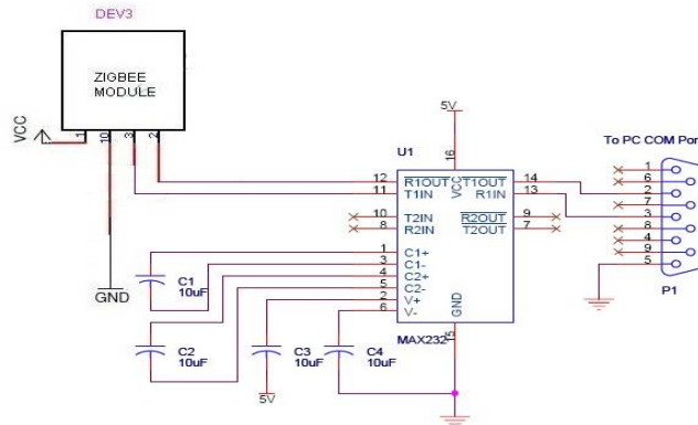
Figure 5. Pc Interfacing circuit
