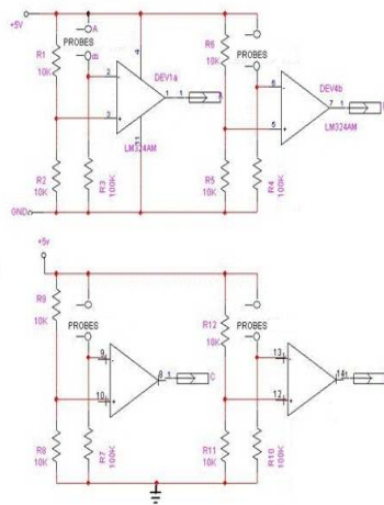
Figure 4. Level Sensor
