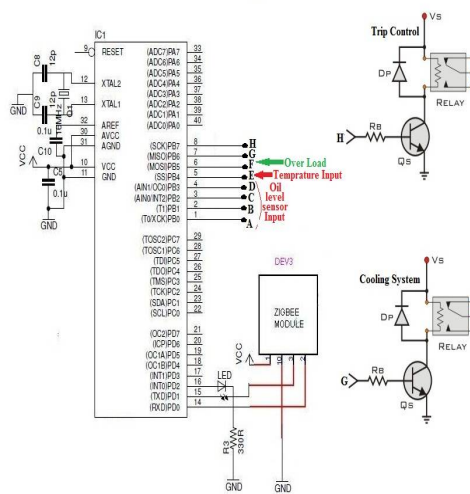
Figure 3. Interface Circuit
