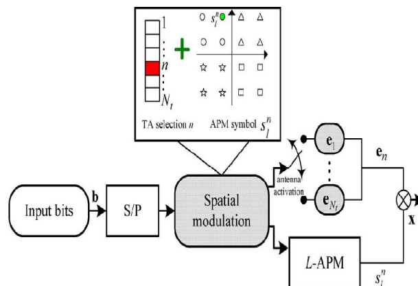
Fig. 1: SM bit-to-symbol mapping rule[5]
