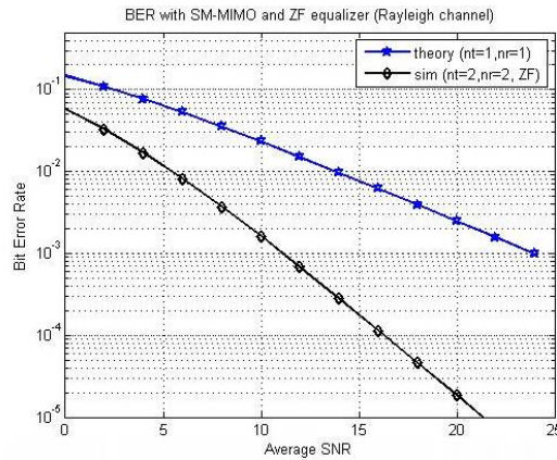
Fig.2. SNR vs BER for n_t = 2, n_r = 2, K=4, n_a = 1
