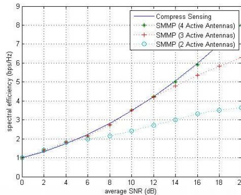
Fig. 3. SNR vs Spectral efficiency
