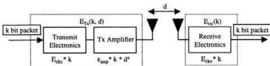
Fig. 2: Radio Model
