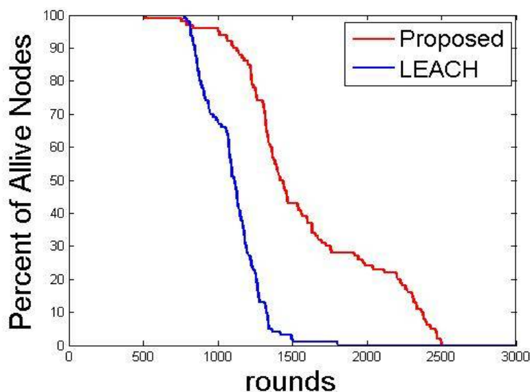
Fig. 3: Interval plot- Analysis of network lifetime
