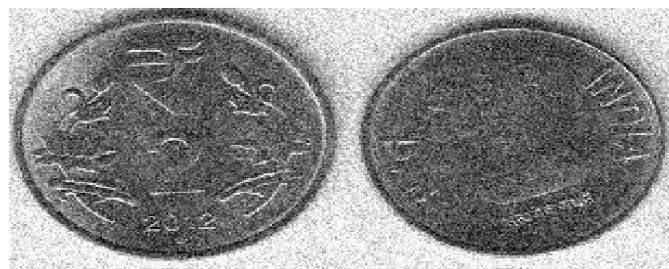
Figure 2: Gaussian noise
