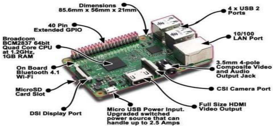
Fig.2 Raspberry Pi3
