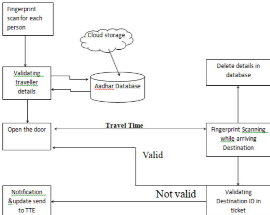
Fig No 1. Architecture Diagram
