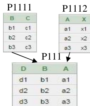
Fig. 3.A - Structure of database in ORACLE to be migrated in MS-EXCEL
