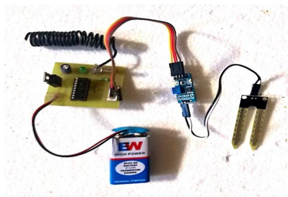
Figure 7: experimental setup for Node3
