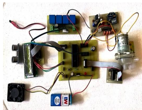
Figure 6: experimental setup for Node2
