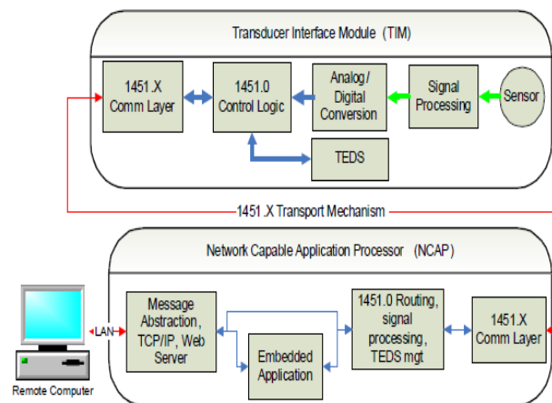
Fig.1. IEEE 1451 smart transducer concept.
