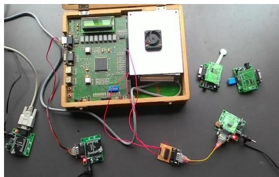
Fig. 6. Hardware physical map.
