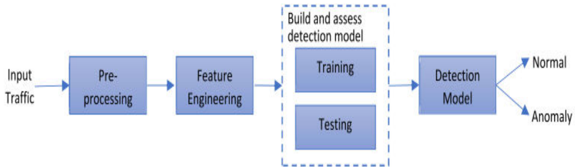
Fig 1: Proposed System
