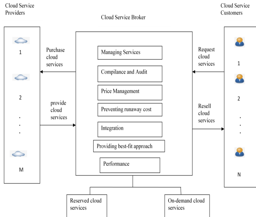
Fig.2 System Architecture
