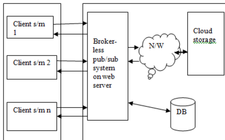
Figure.1. System architecture
