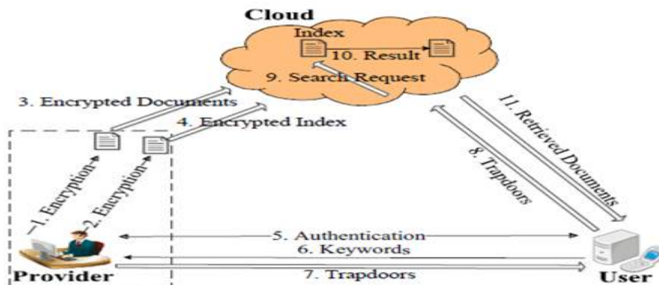
Figure 1: Traditional Encryption search system over cloud
