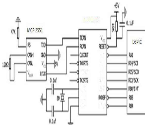
Fig.3 CAN Interface Module
