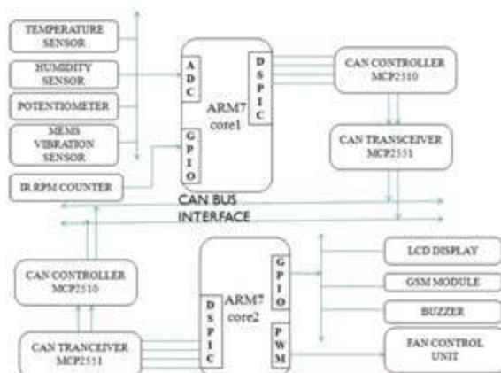
Figure 1: Block diagram of Processing Module
