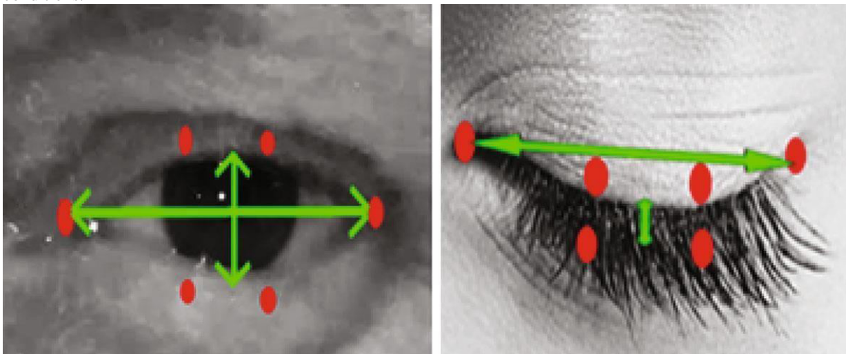
Fig.1 : Eye landmarks
