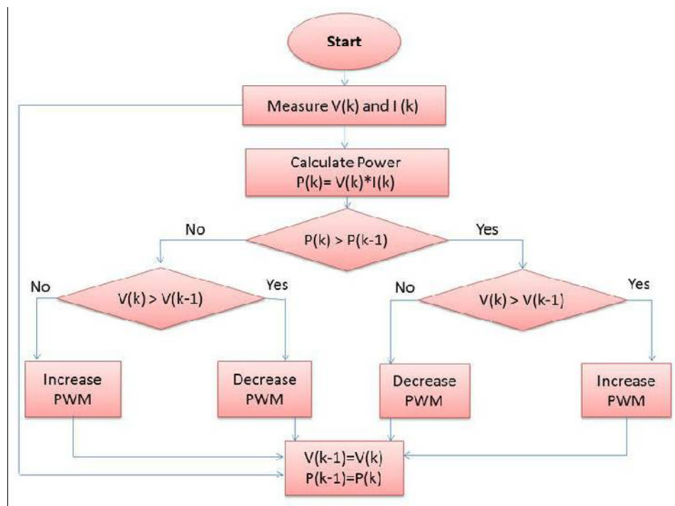
Figure 5. Algorithm
