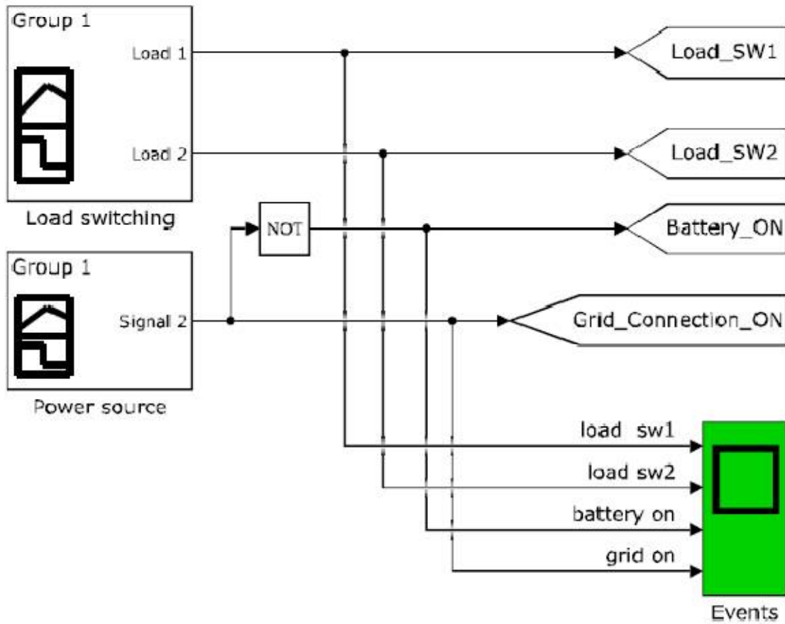
Figure 8. Simulation block of output
