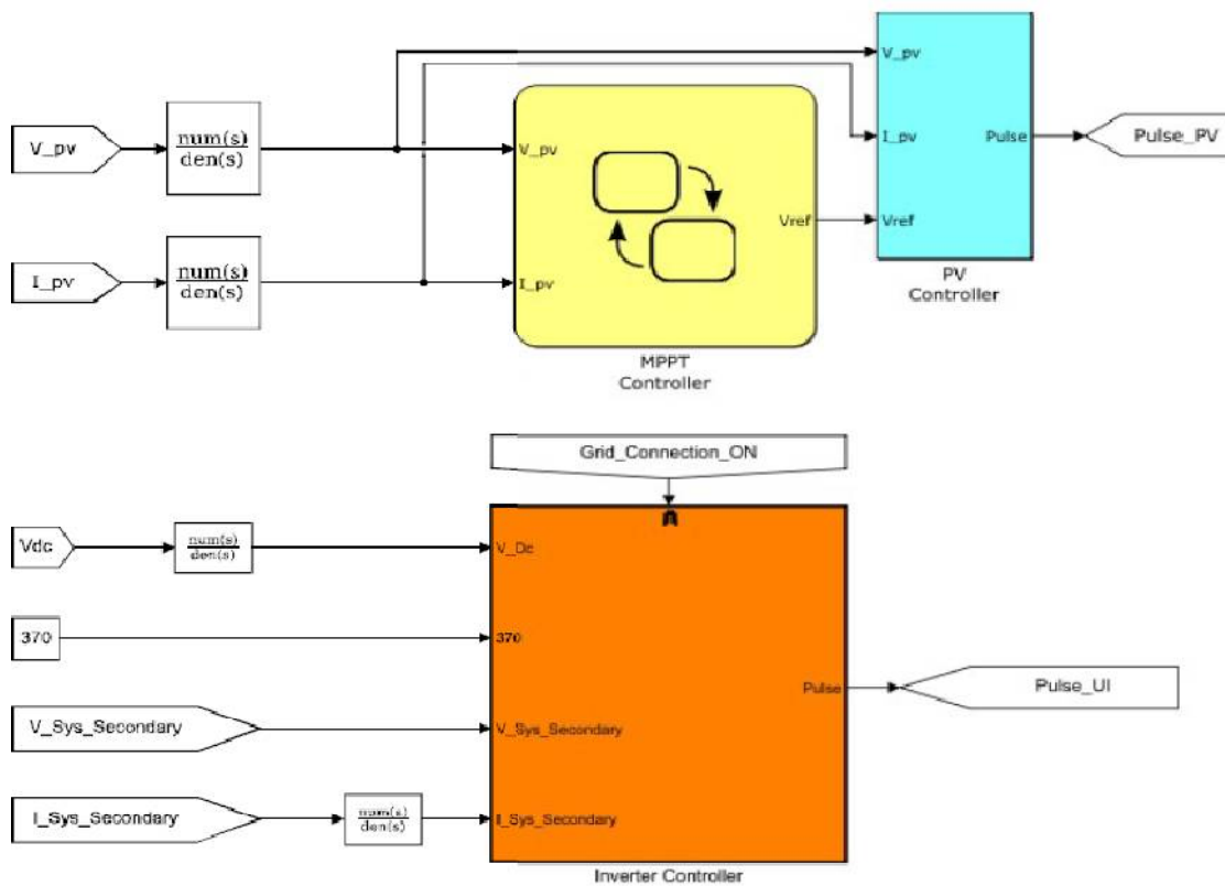
Figure.7. Simulation block of MPPT
