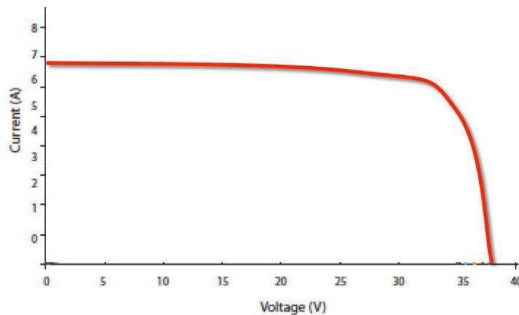
Figure 1: Standard PV I-V Curve
