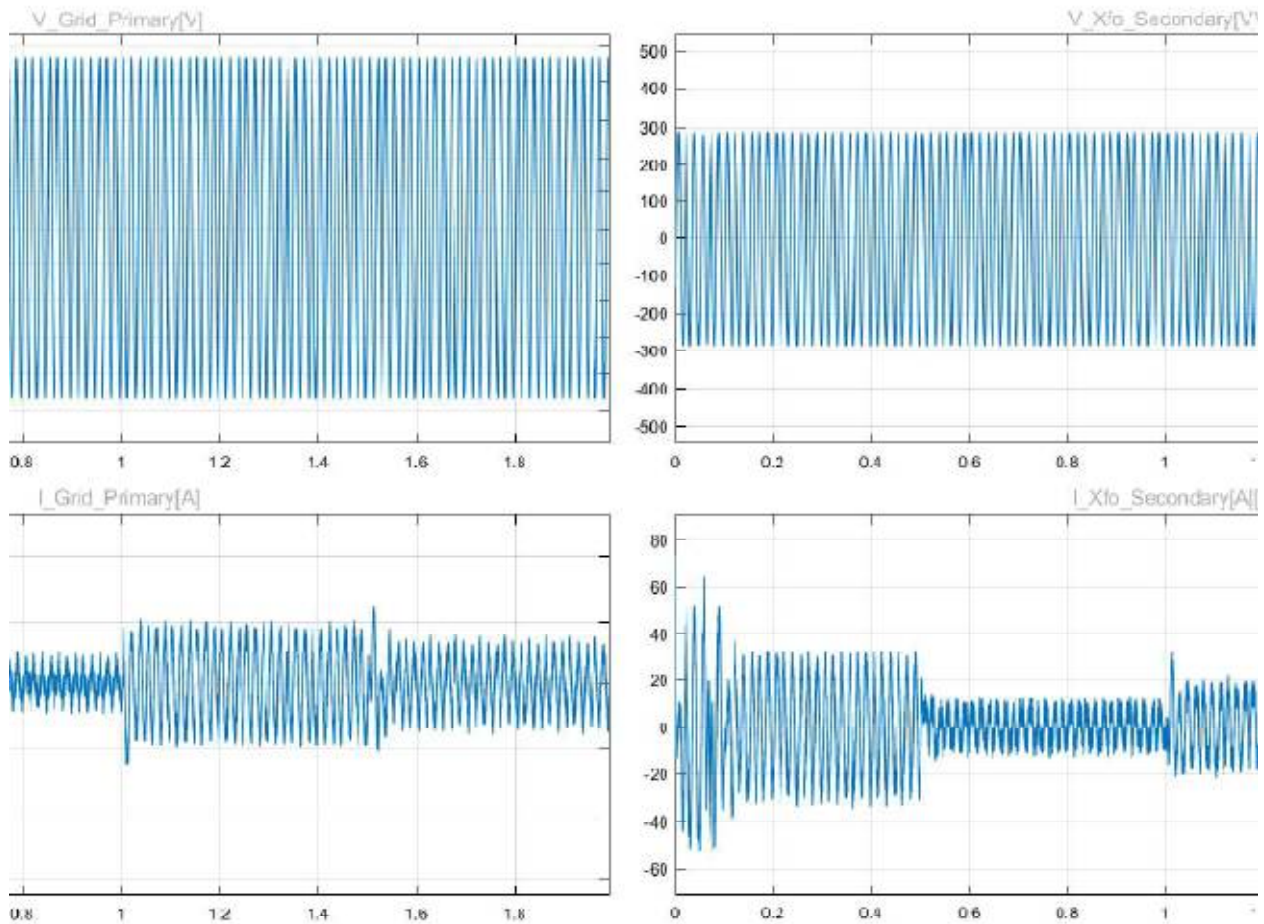
Figure .11. Grid side output
