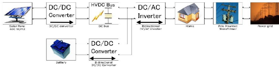
Figure 6. Simulation of single phase grid connected inverter using MPPT
