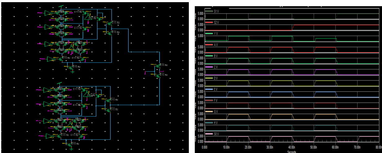
Fig.6 ECRL 8X1 Multiplexer Schematic design and output wave form
