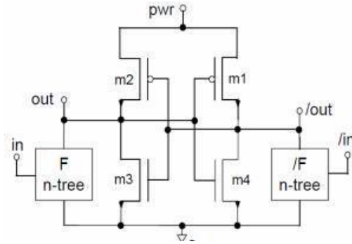
Fig. 3. 2N2N2P Schematic
