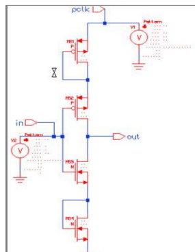
Fig. 5. Proposed Logic Inverter Schematic
