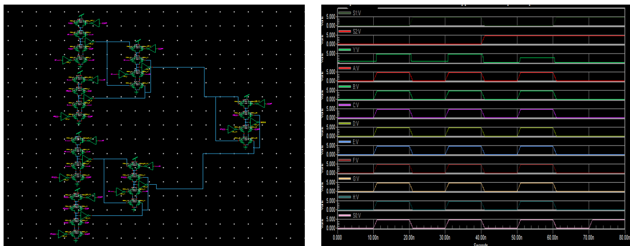
Fig.8 2N2N2P 8X1 Multiplexer Schematic design and output wave form
