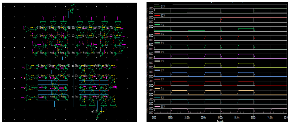
Fig.10 Proposed 8X1 Multiplexer Schematic design and output wave form
