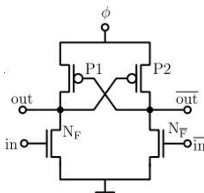
Fig. 2. ECRL Buffer/Inverter Schematic
