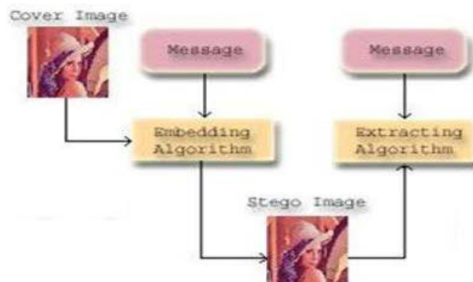
Figure 2. Image Steganography
