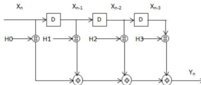
Figure 1: 4-tap FIR Filter
