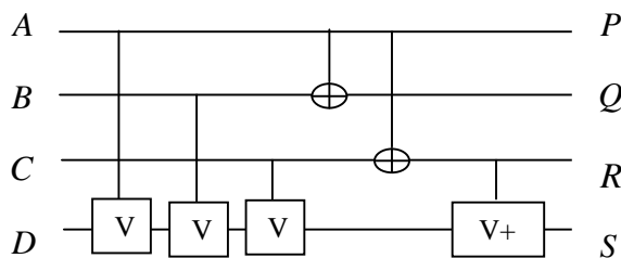
Figure 5: Quantum Representation of the HNG Gate
