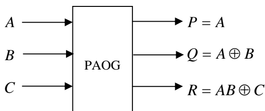
Figure 6: Block Diagram of the PAOG
