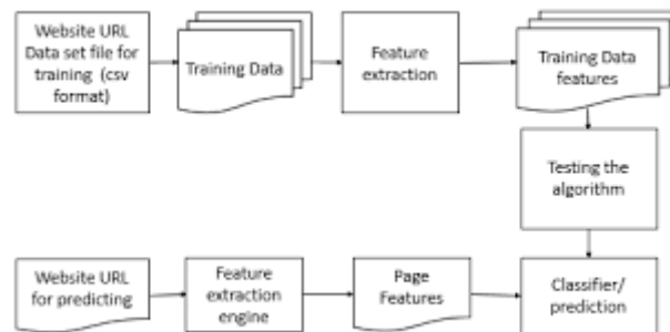
Fig 1. Block diagram for detecting suspicious URL
