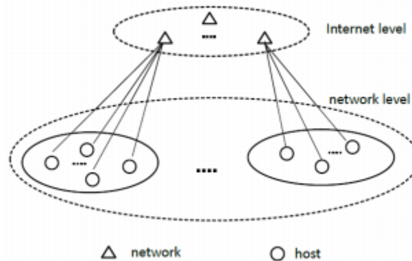
Figure 1: The two layer network structure used to create the large-scale network for studying malware propagation.
