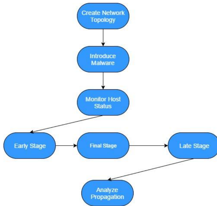
Figure 2: The flow of how the idea is executed and malware propagation is analyzed.
