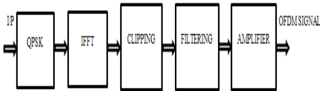
Figure 2. OFDM signal transmission block diagram with ACF
