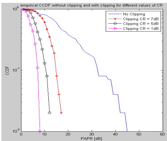
Figure 5. Empirical CCDF without clip and with clipping and filtering
