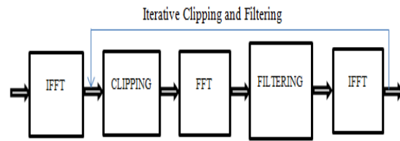
Figure 3. OFDM signal transmission block diagram using ICF
