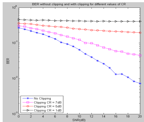
Fig.6. .BER without clipping and with clipping and filtering
