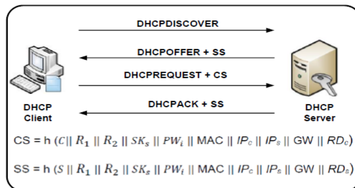
Figure 3: the DHCP message exchange using MA technique
