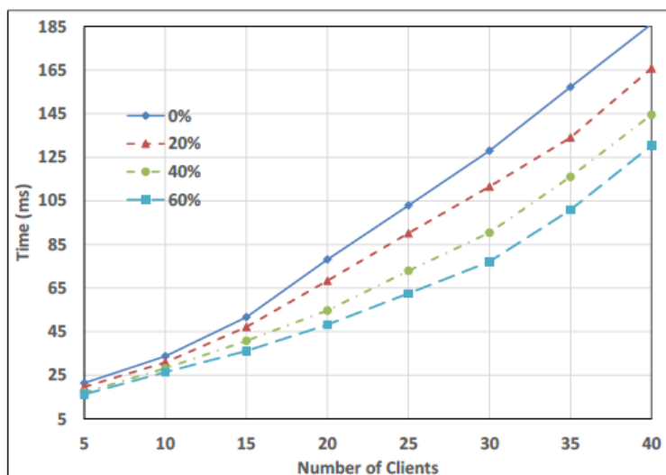
Figure 4: MAT versus N with increasing number of attackers
