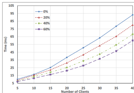
Figure 3: CAT versus N with increasing number of attackers
