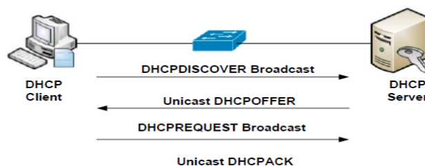
Figure 1: DHCP protocol operations
