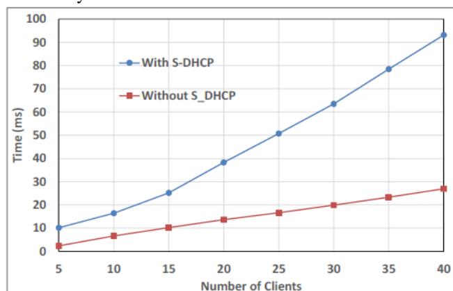
Figure 6: MAT versus N with in the case of using DHCP and S-DHCP
