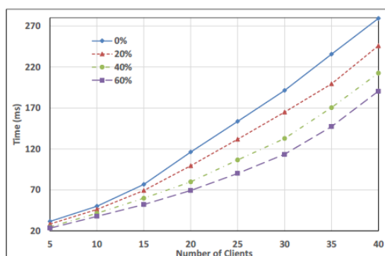
Figure 5: CT versus N with increasing number of attackers
