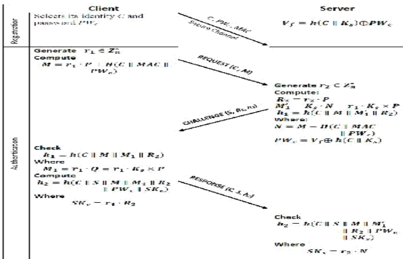
Figure 2: Flow diagram for EAKM technique
