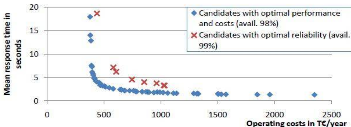
Fig. 2. PerOpteryx Results of BRS Design Space Exploration
