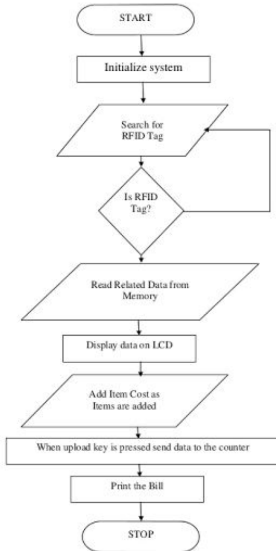
Fig. 2. Flowchart of proposed system
