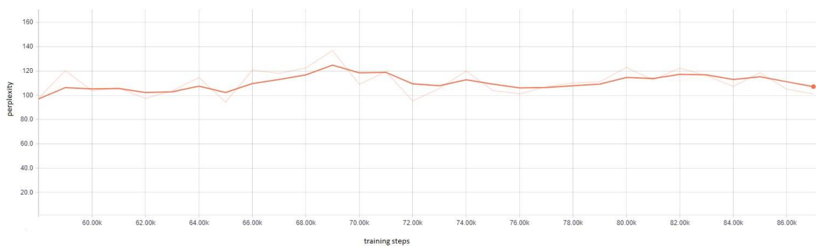
Figure 4: Test perplexity
