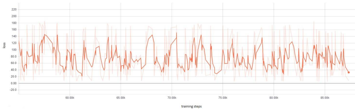
Figure 3: Training loss
