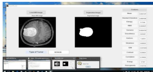
Fig.4 Binary Image
