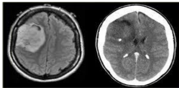
Fig.3 Gray Image
