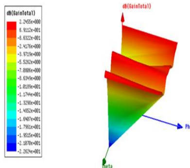
Figure(6)Measured Gain
