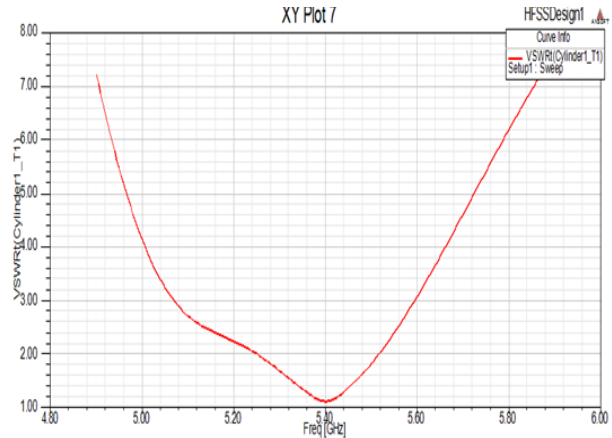
Figure(5)Measured VSWR
