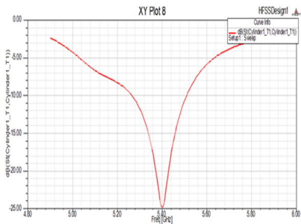
Figure(4)Measured Return Loss
