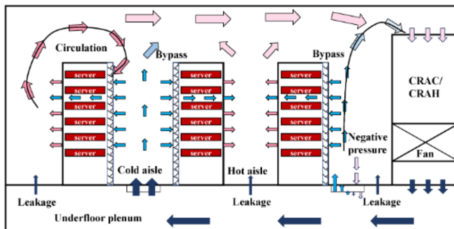
Figure 1: Diagram of room-level air cooling.
