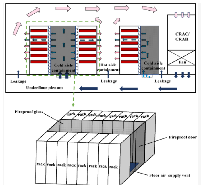
Figure 2. Diagram of cold aisle containment in the computer room.
