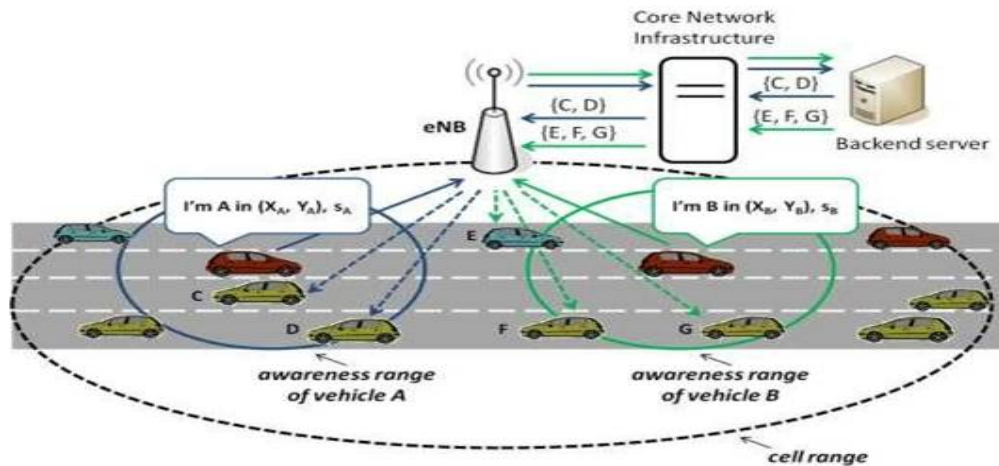
Fig. 1. Multicast CAM delivery in LTE. The awareness range of the vehicles does not coincide with the cell range.
