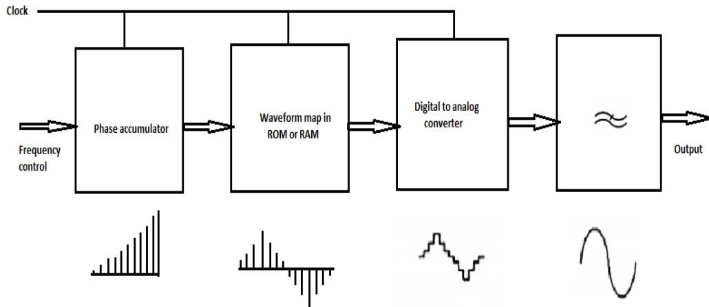
Fig. 3. DDS Block Diagram and Waveforms
