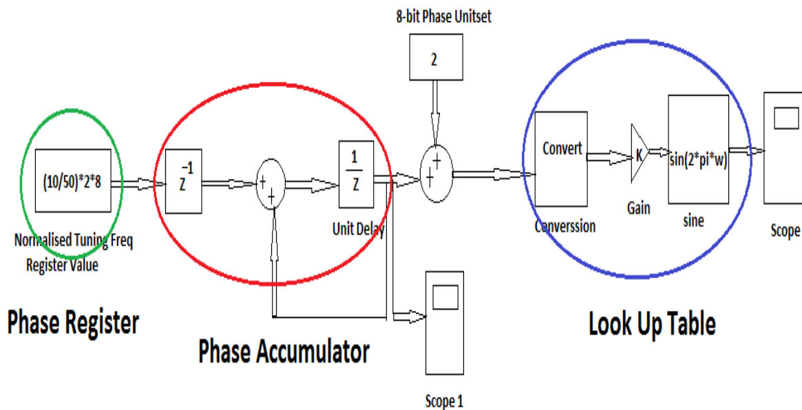
Fig. 4. MATLAB Simulink Model of DDS
