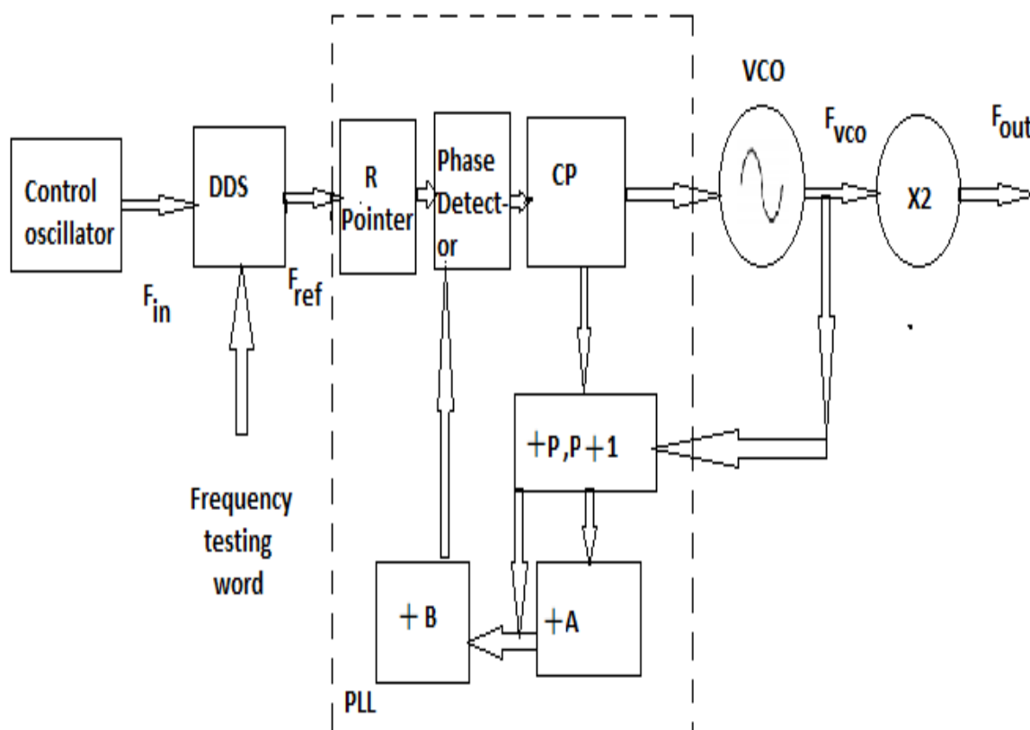
Fig. 5. Block Diagram of the DDS driven PLL Frequency Synthesizer
