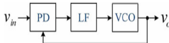
Fig. 1. Basic PLL Structure
