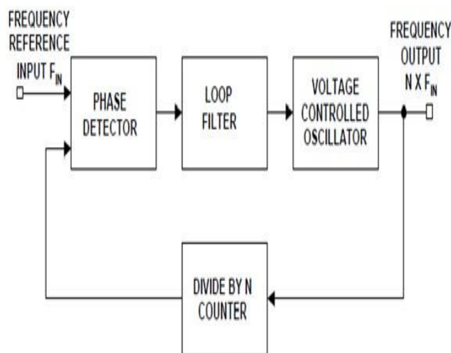
Fig. 2. Standard PLL Structure
