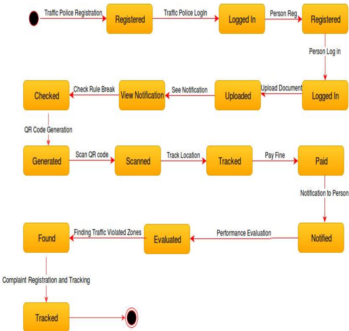
Figure 2. Flow diagram (Methodology) of proposed system
