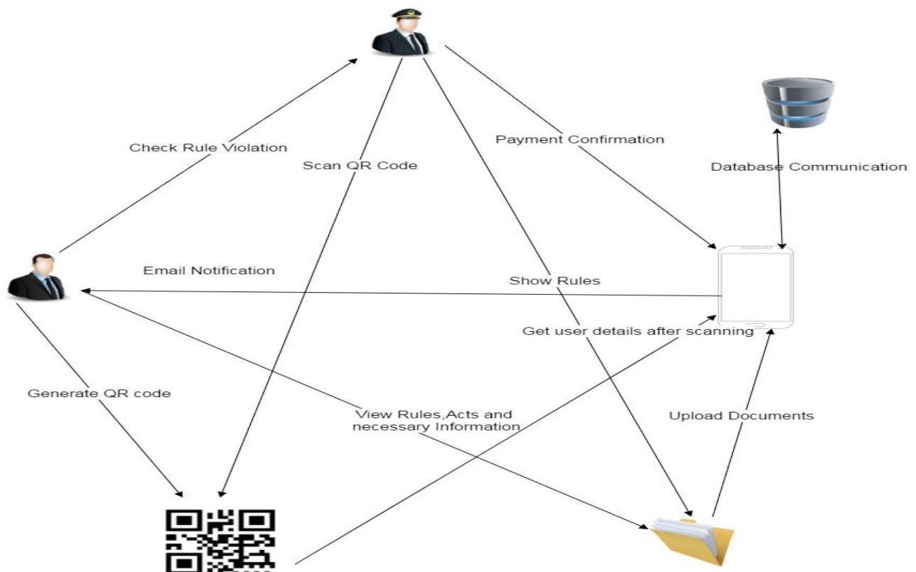
Figure 1. Architecture diagram of proposed system
