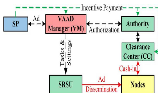
Fig: 3. Overview of VAAD
