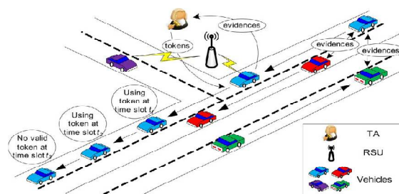
Fig. 4. Evidence-token mechanism.
