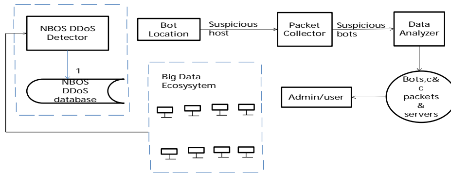
Fig:Architecture Diagram for Botnet
