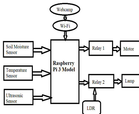
Fig1: Irrigation Control System (Transmitting Section)
