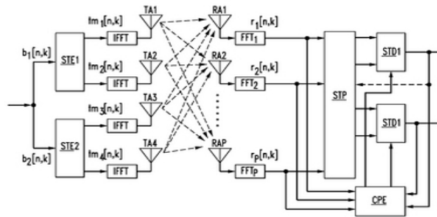
Figure 1: Block Diagram of MIMO-OFDM
