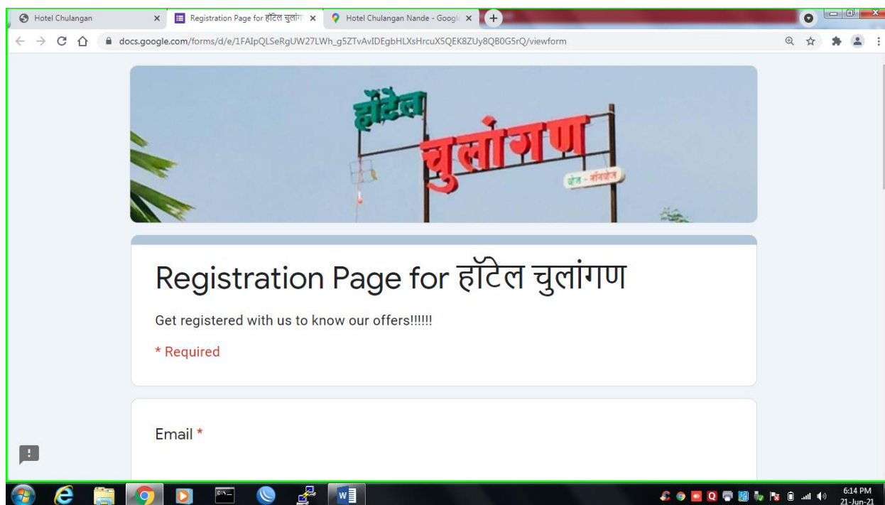
Fig.2: Registration Page
