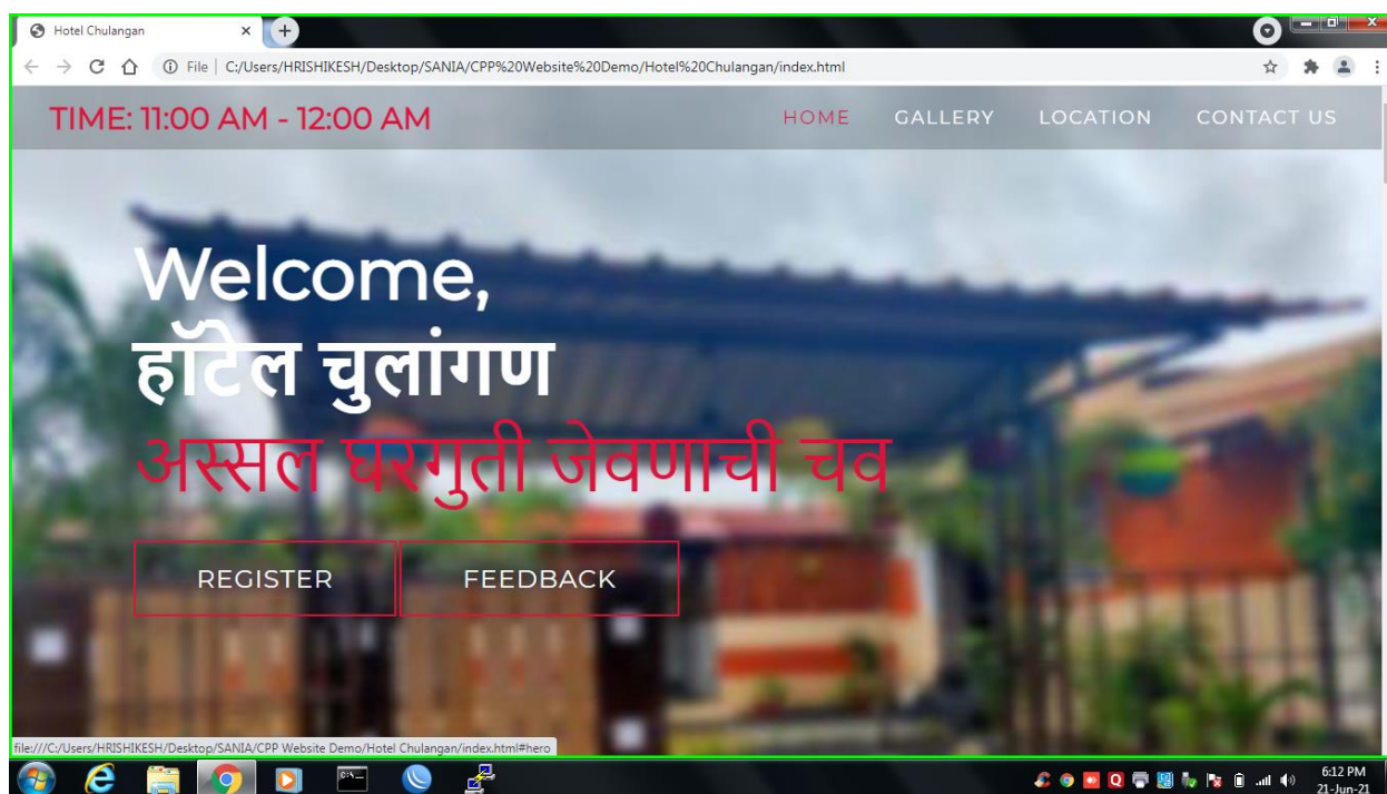
Fig. 1: Home Page
