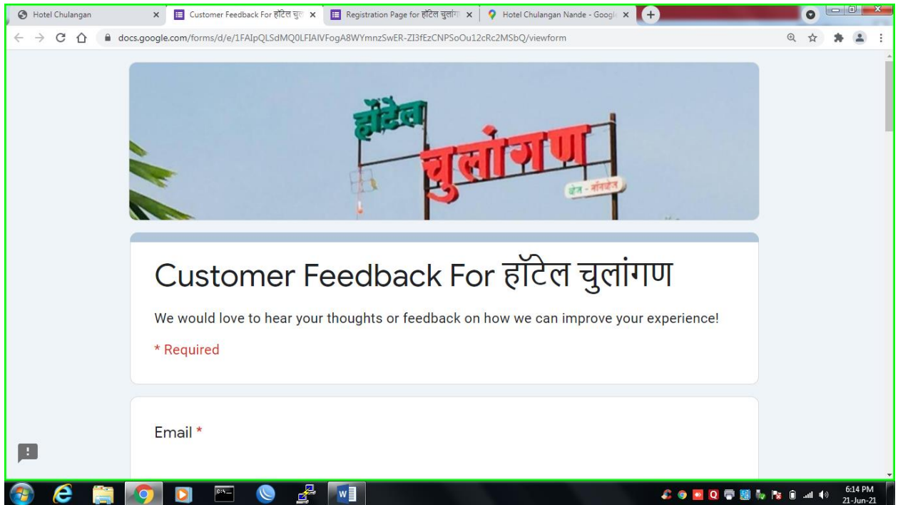
Fig. 3: Feedback Page
