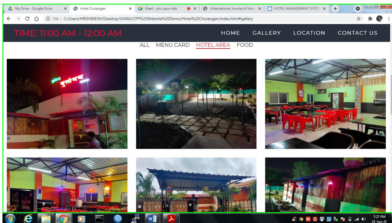
Fig. 5: Gallery Page-2
