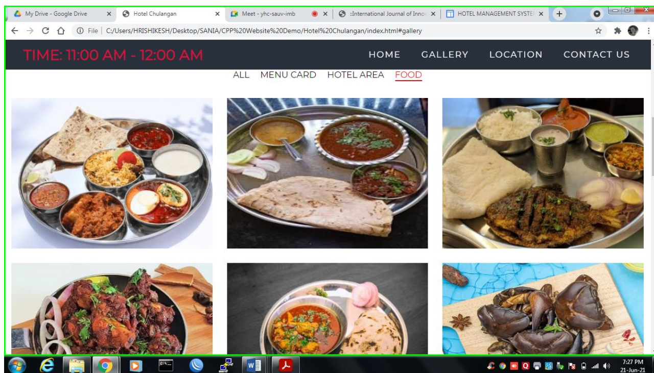
Fig. 6: Gallery Page-2
