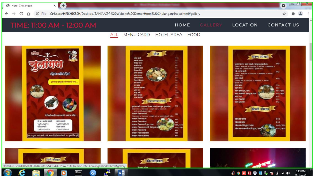
Fig. 4: Gallery Page-1
