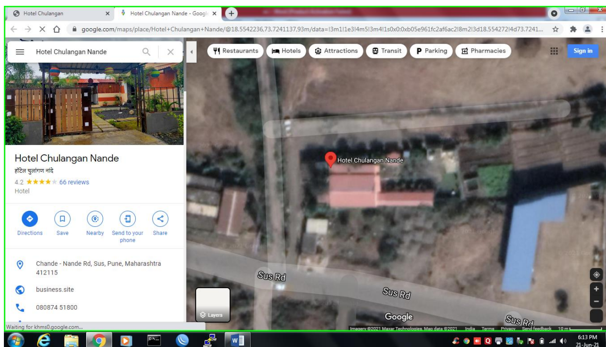
Fig.7: Location Page
