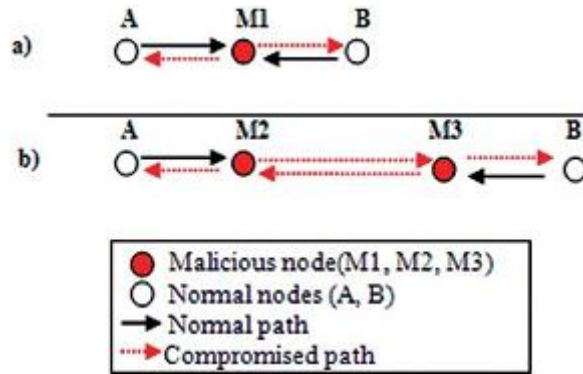
Figure 1. malicious node detection
