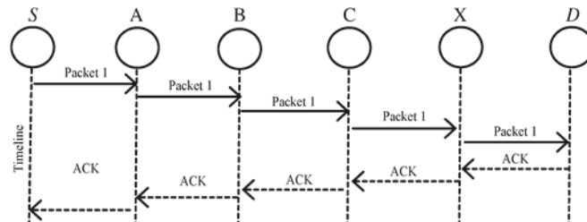
Fig.4 ACK scheme: The destination node is required to send acknowledgment packets to the source node.
