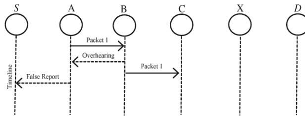
Fig. 7.False misbehavior report: Node A sends back a misbehavior report even though node B forwarded the packet to node C.
