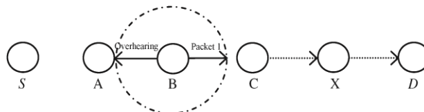
Fig. 6. Limited transmission power: Node B limits its transmission power so that the packet transmission can be overheard by node A but too weak to reach node C.
