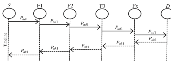
Fig. 8 System control flow: This figure shows the system flow of how the EAACK scheme works.
