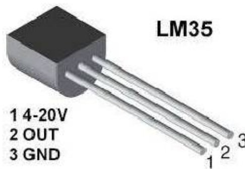
Fig 5: Temperature Sensor
