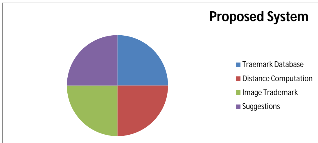
Fig 2: System Graph
