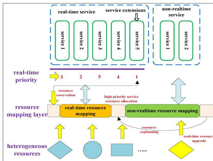
Fig1.Allocation of Resource in Service Oriented System
