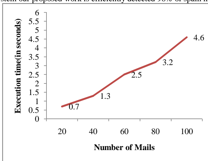
Fig 6. Execution Time of e- mail Abstraction Generation of the System
