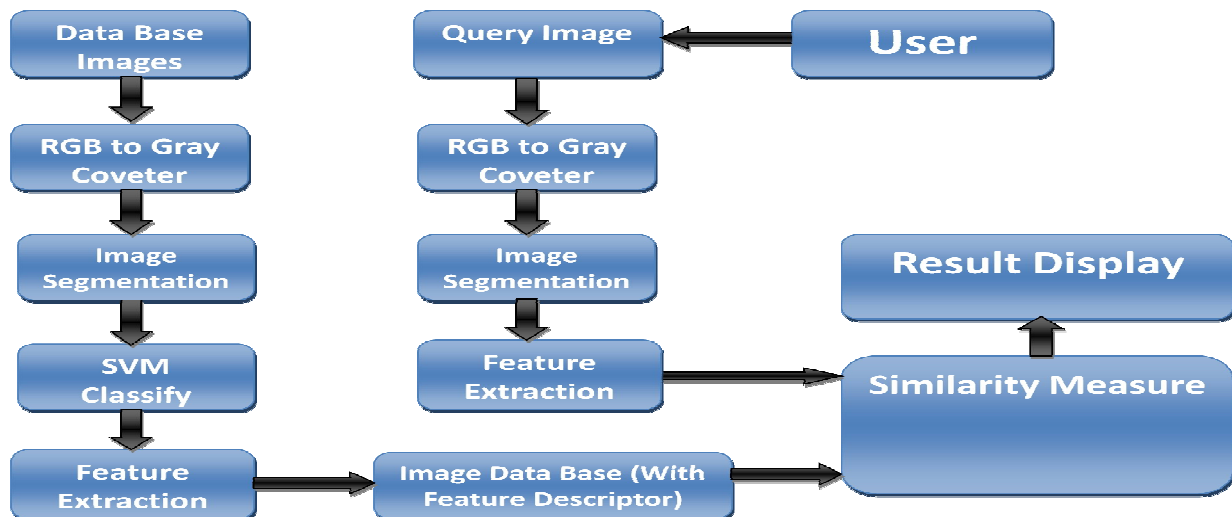
Fig.2:Block Diagram of Proposed Method
