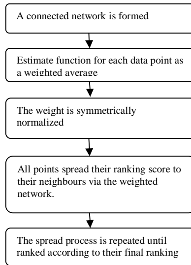
Fig.3: Algorithm Flow Chart
