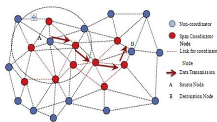
Fig. 3. Route Discovery of EASRP
