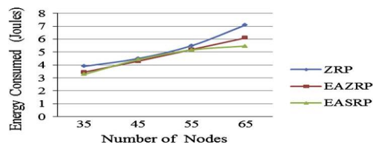
Fig. 5. Average consumed energy
