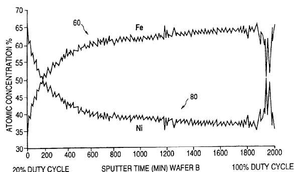
FIGURE 1: Atomic concentration of Fe, Ni in a magnetic disk
