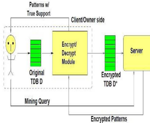
Fig 1:Architecture of Existing System
