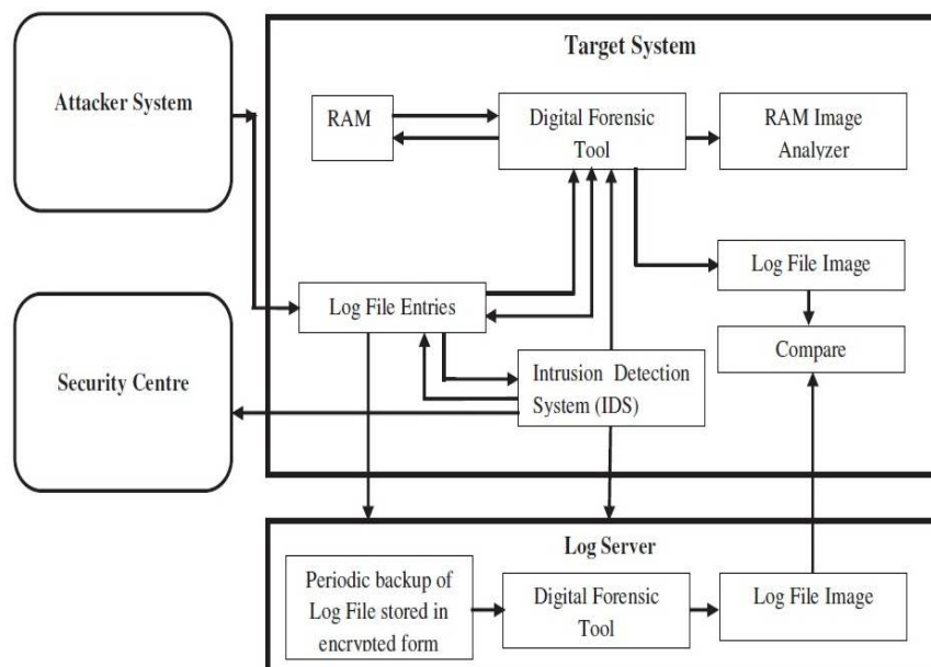
Fig.2. Flow of System
